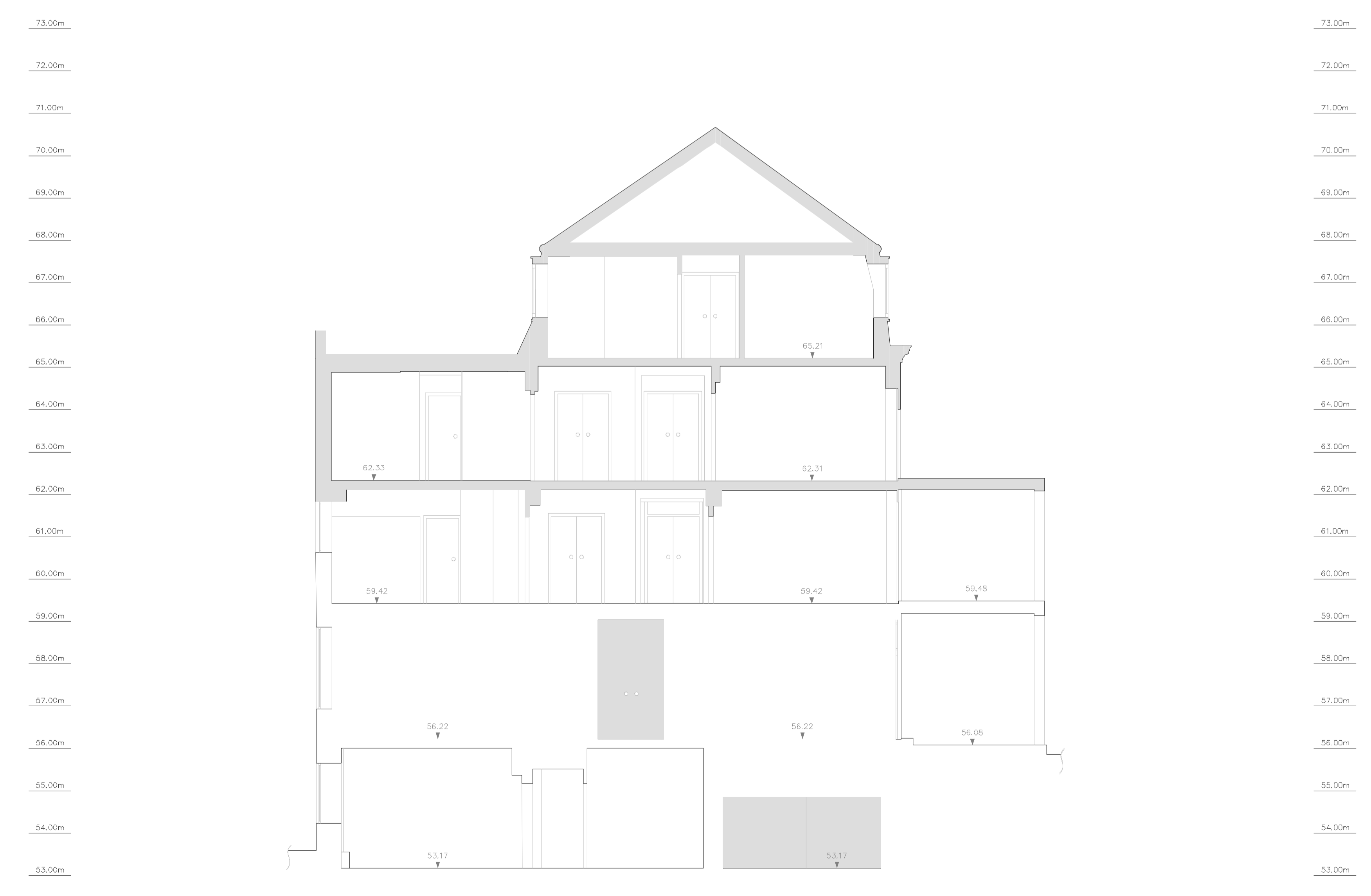
EXISTING SECTION B-B
